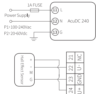
Power Supply Wiring
