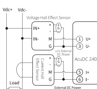
Voltage & Current Wiring using Hall Effect Sensors
