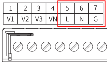
Fig. 2-5 Power Supply Wiring
