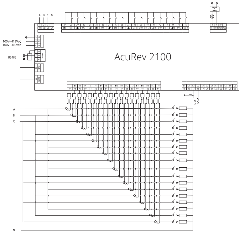
Fig. 2-6b Single Phase Option 2
