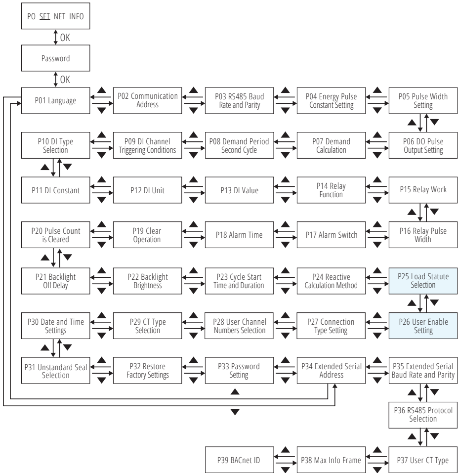
Fig. 3-20 Basic Settings
