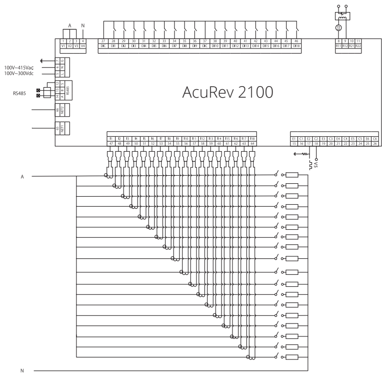
Fig. 2-6a Single Phase Option 1
