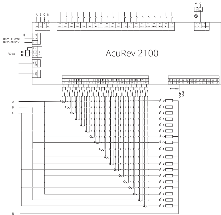
Fig. 2-9 Three-Phase Three-Wire (2LL)
