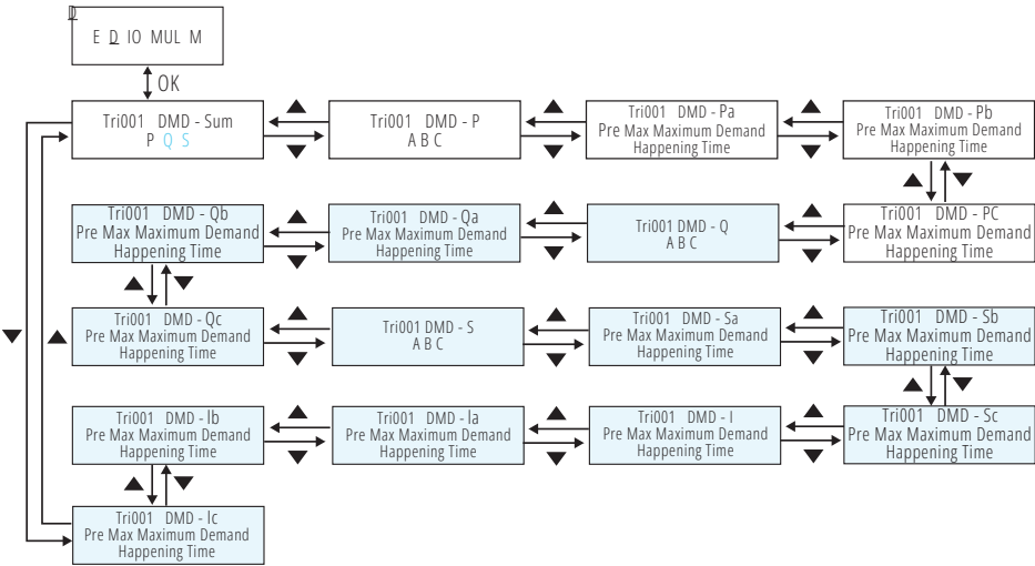
Fig. 3-9 Three Phase 4 Wire Demand Display
