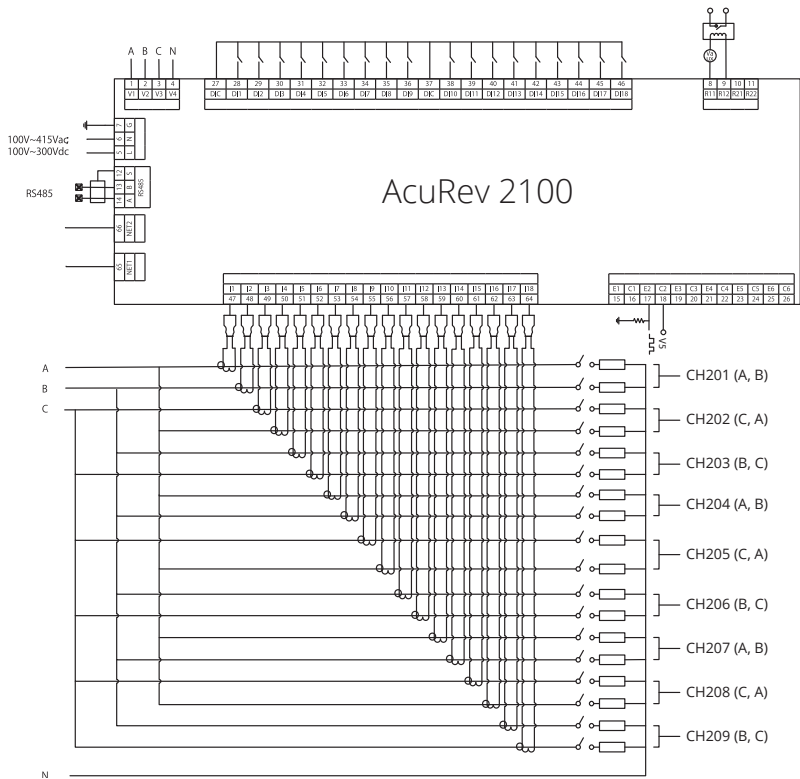
Fig. 2-10 Network Wiring
