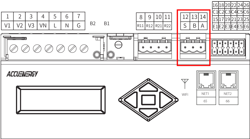
Figure 2-11 Communication Port
