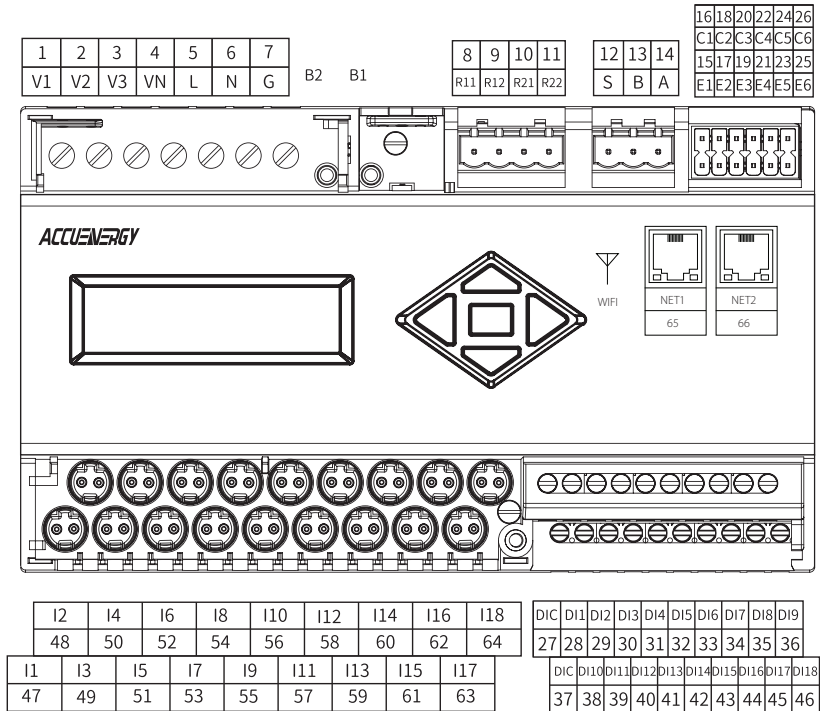
Fig. 2-4 AcuRev 2100 Terminals
