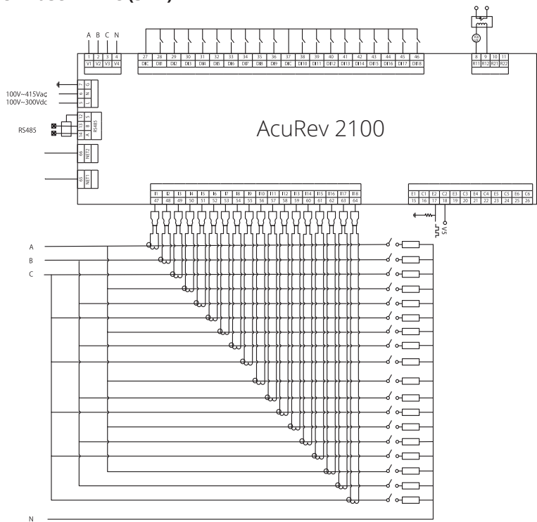
Fig. 2-7 Three-Phase Four-Wire
