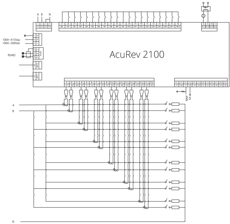
Fig. 2-8 Single Phase 3-Wire (2LN)
