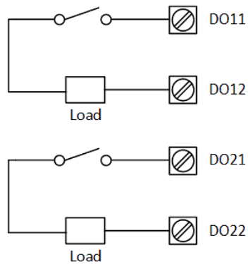
Figure 2-29 DO Connections
