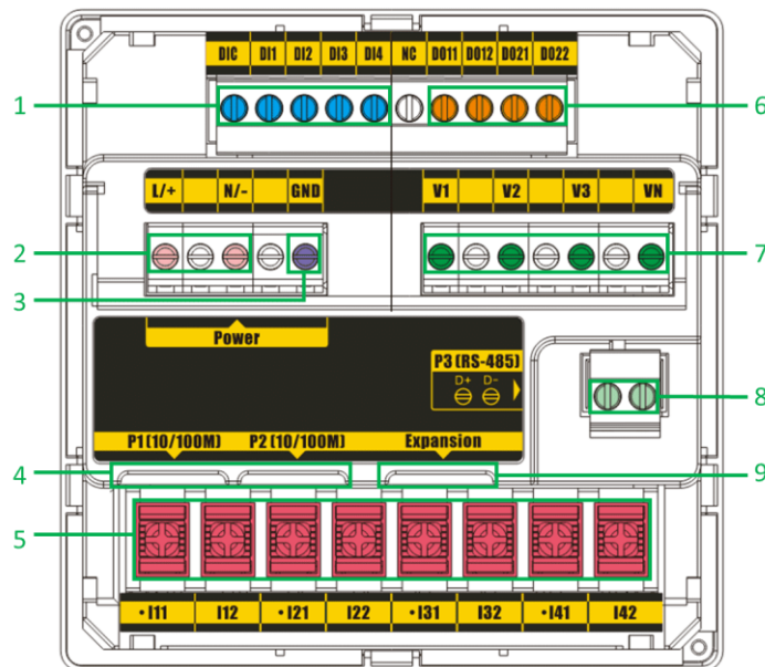
Figure 2-1 Appearance
