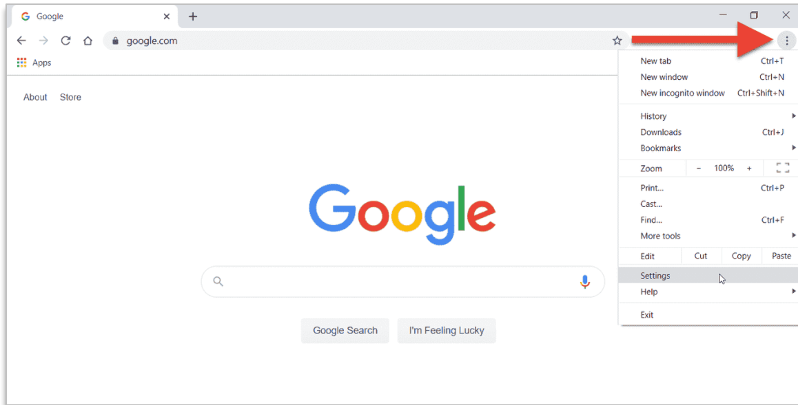
Figure 3-52 Chrome Settings
