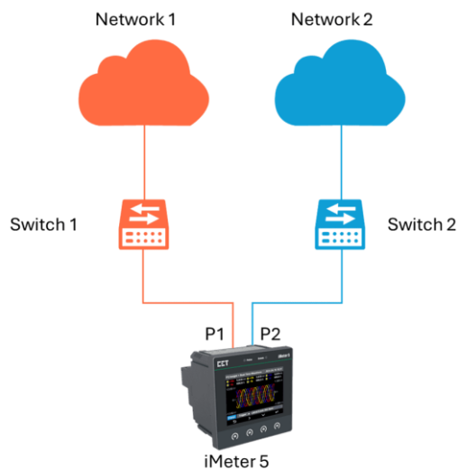
Figure 2-23 Ethernet Normal Mode and Switch Mode
