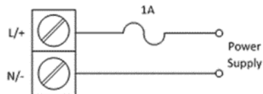
Figure 2-31 Power Supply Connections
