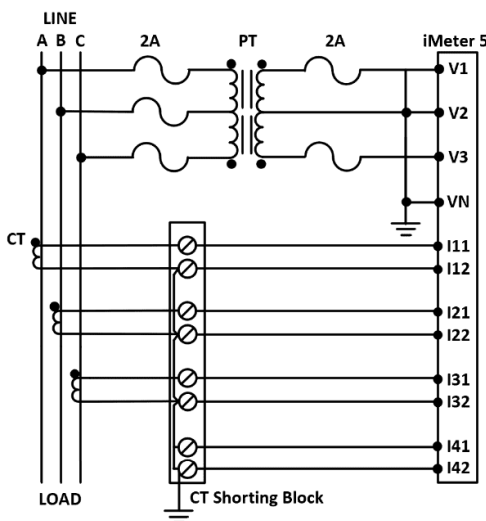
Figure 2-18 3-Phase 3-Wire Open Delta with 2PTs & 3CTs
