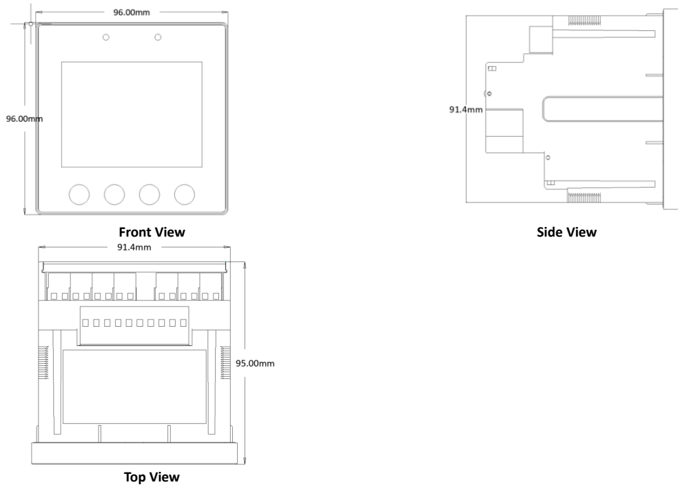
Figure 2-3 Dimensions
