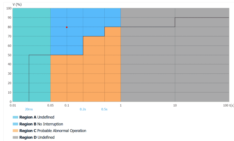
Figure 4-18 SEMI F47 Plot Descriptions
