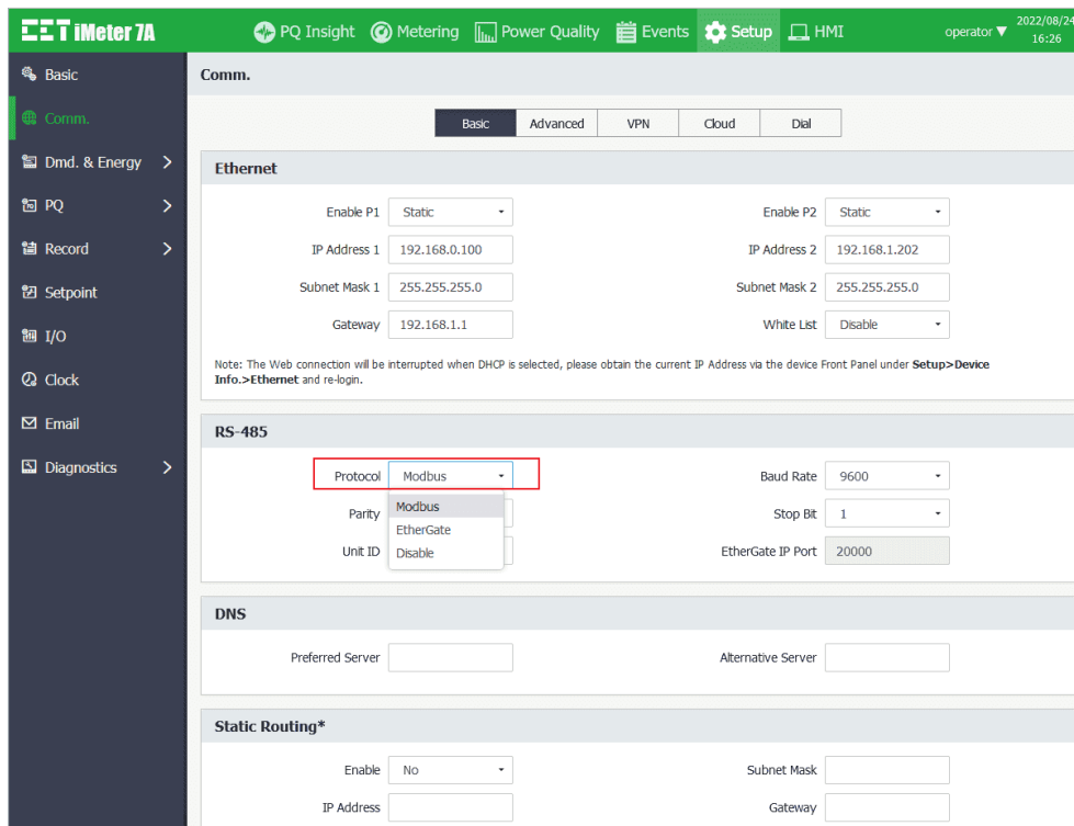
Figure 4-44 Select "EtherGate" Mode on the Web Server
