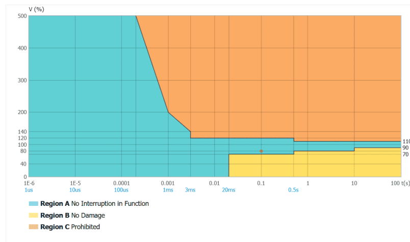
Figure 4-17 ITIC Plot Descriptions
