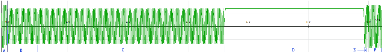
Figure 4-28 An Example of DWR
