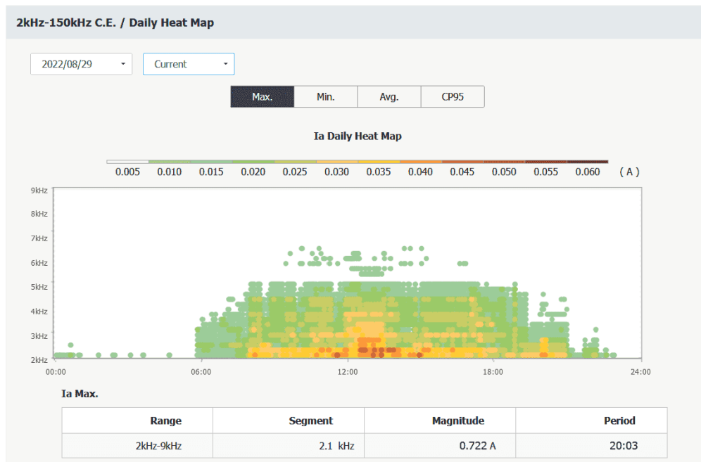
Figure 4-15 Daily Heat Map for Ia Max.
