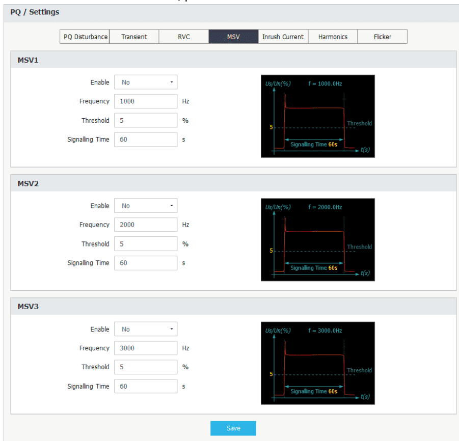
Figure 3-141 MSV Settings Interface
