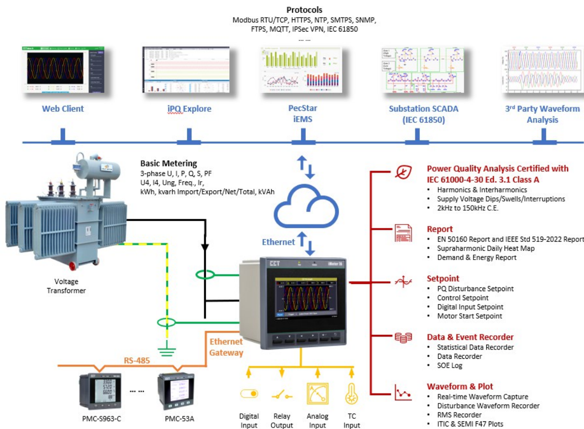
Figure 1-1 Typical Application
