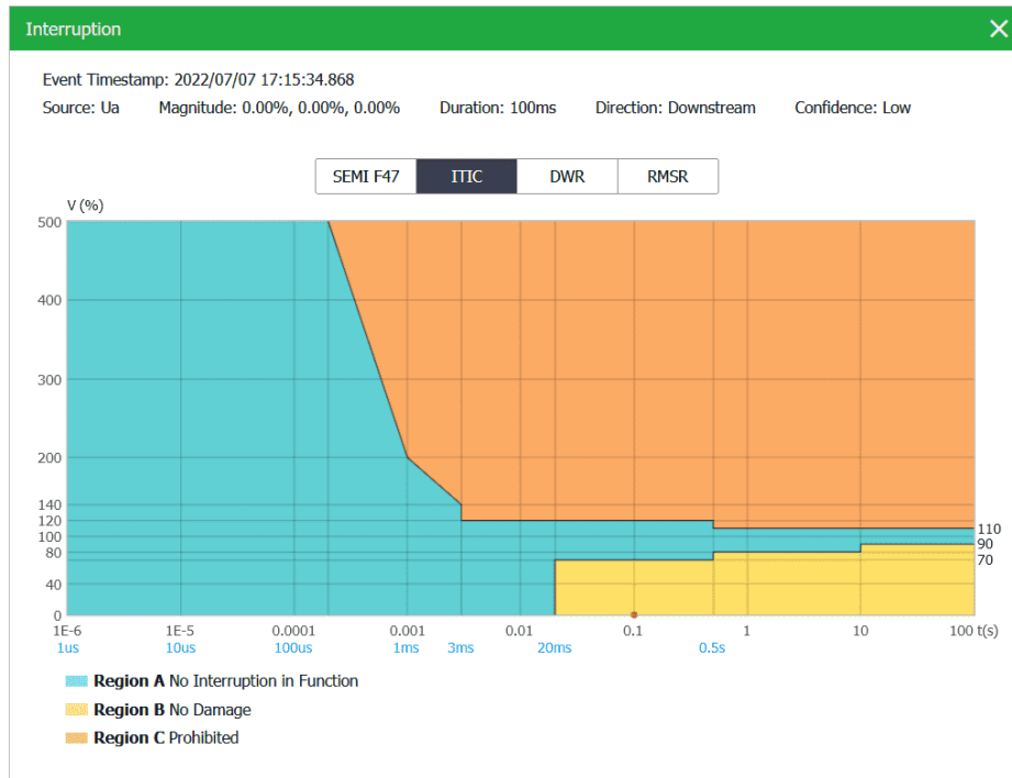
Figure 3-113 Interruption on ITIC Interface
