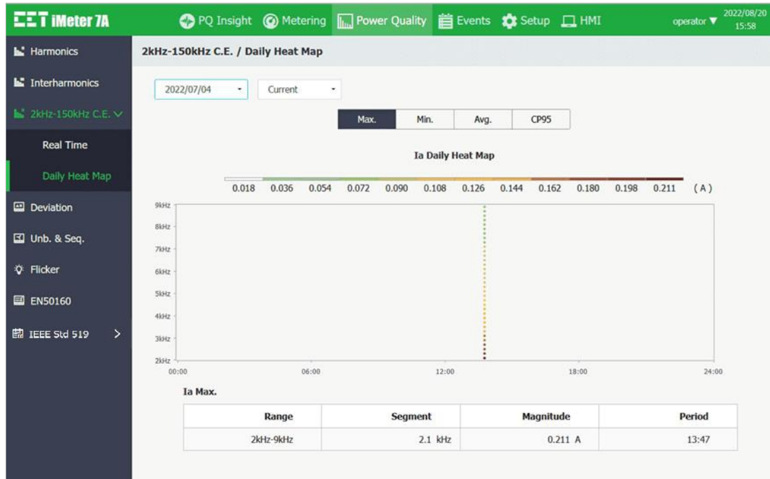
Figure 3-88 Daily Heat Map – Peak value for Ia Max.
