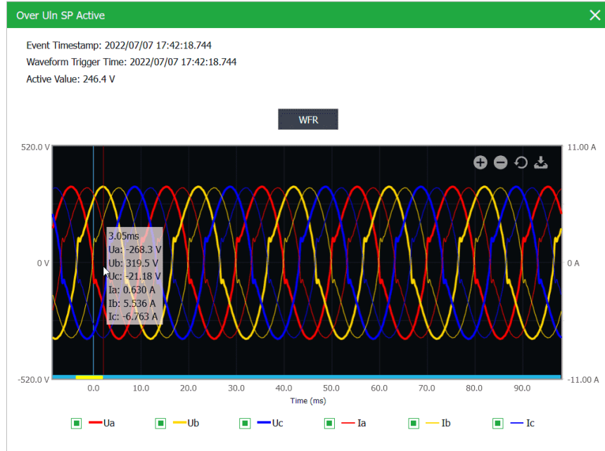
Figure 3-111 Over Uln Setpoint Active
