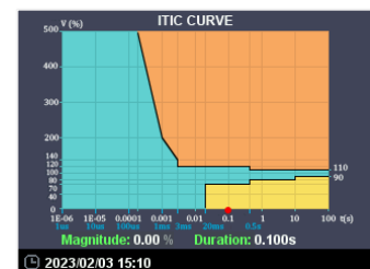
ITIC Curve
