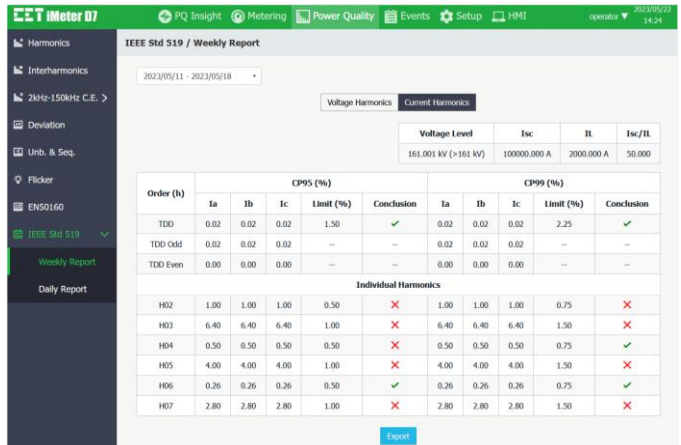
IEEE Std 519-2020 Weekly Current Harmonic Compliance Report
