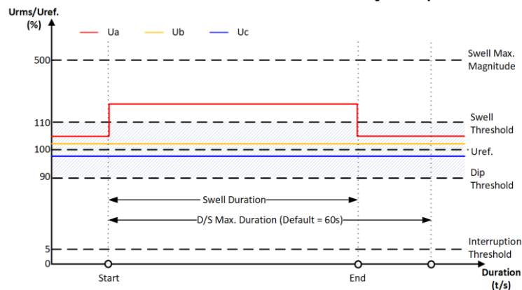
Figure 4-3 Swell Detection Criteria
