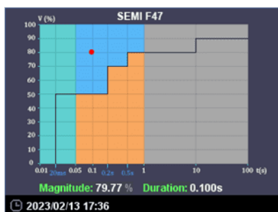
SEMI F47 Curve
