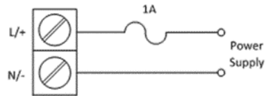
Figure 2-34 Power Supply Connections
