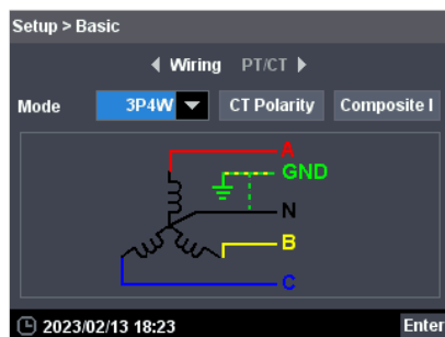
Wiring Setup
