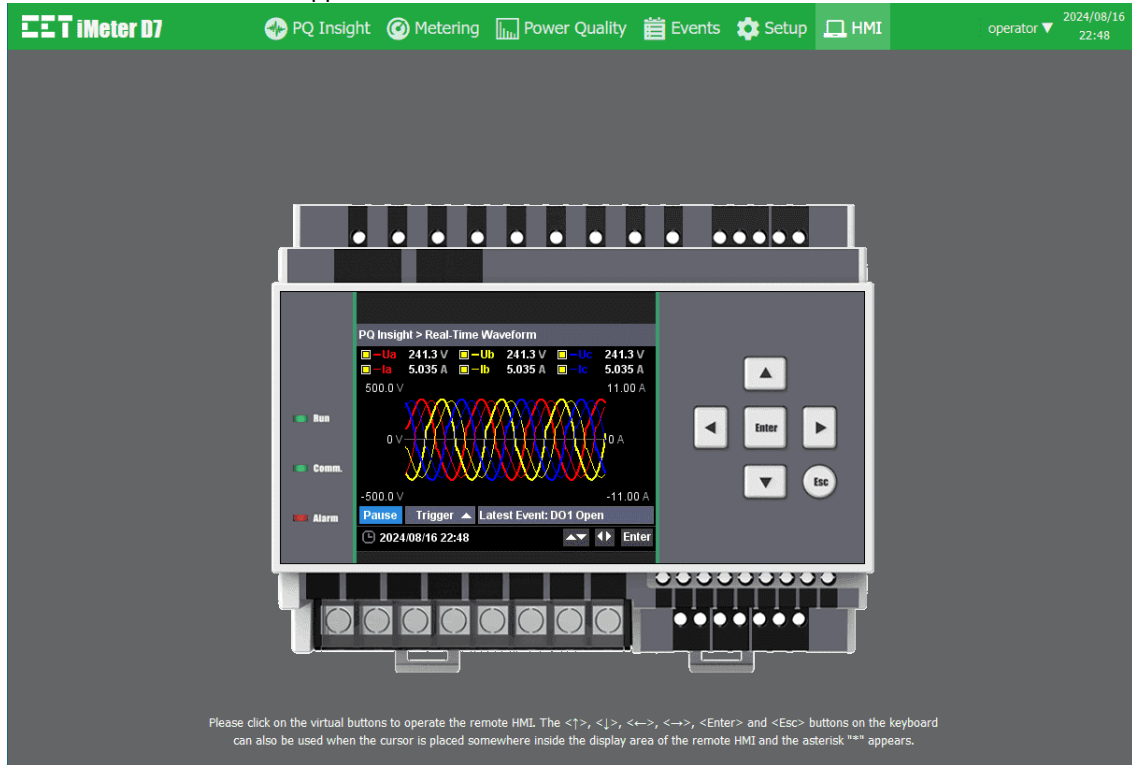
Figure 3-176 HMI Interface
