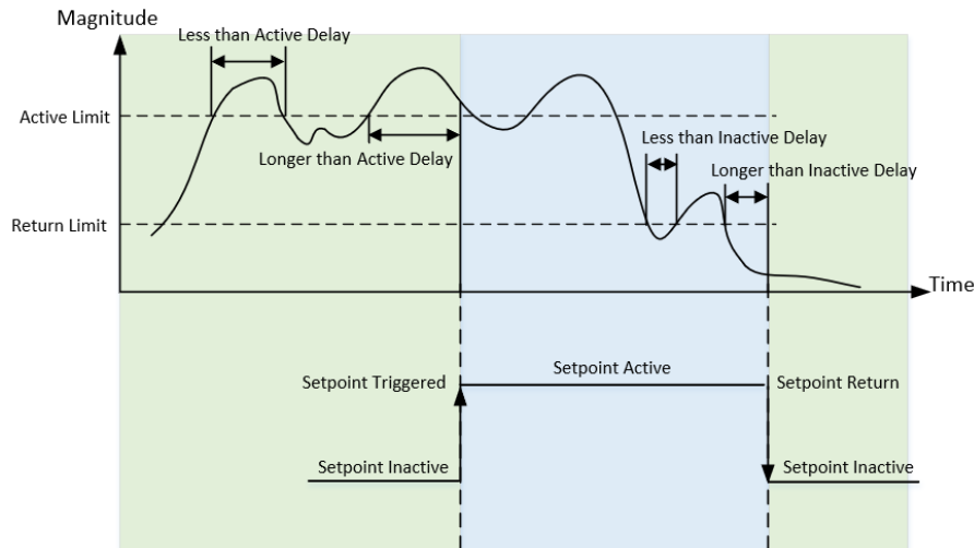
Figure 4-25 Over Setpoint
