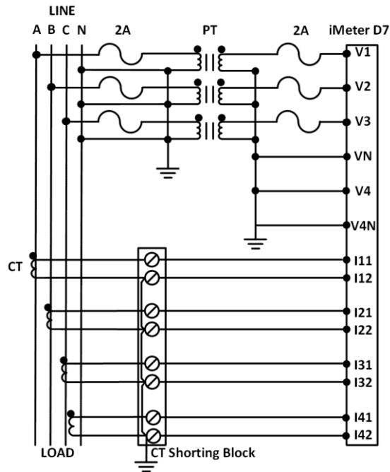
Figure 2-18 3-Phase 4-Wire Wye with 3PTs & 4CTs
