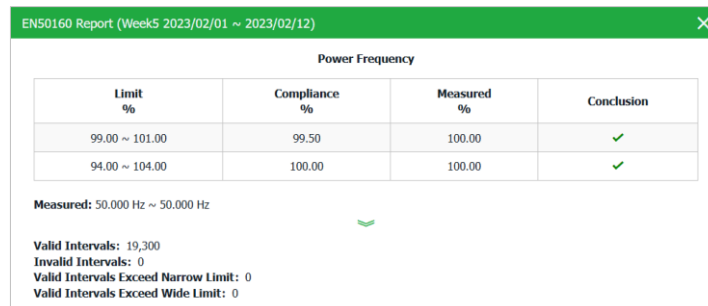
Figure 3-87 Power Frequency
