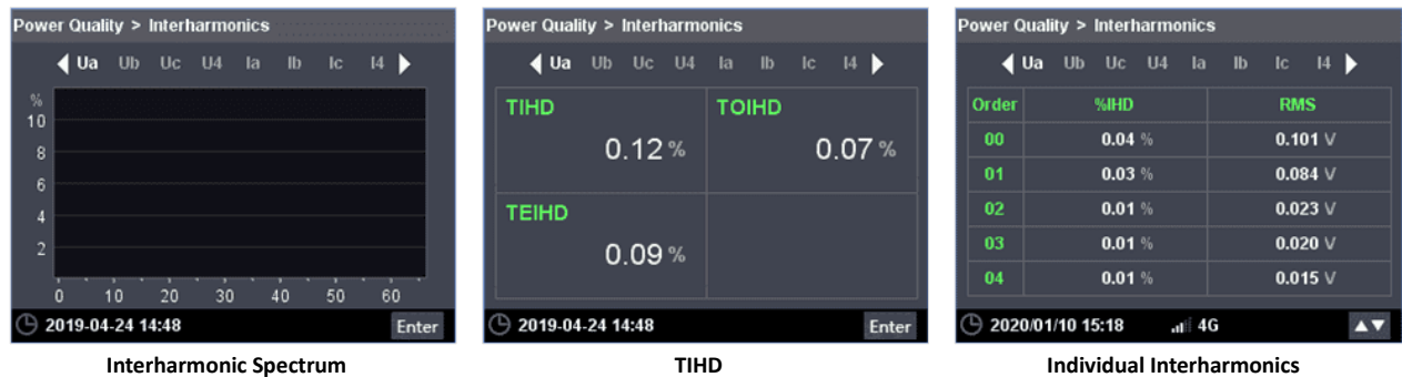
Figure 3-20 Interharmonics
