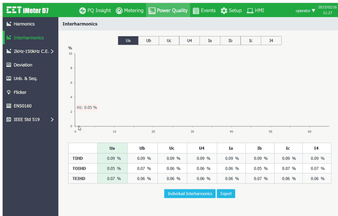
Figure 3-79 Interharmonics Interface
