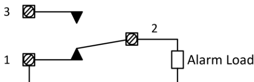
Figure 2-29 Alarm Output Wiring
