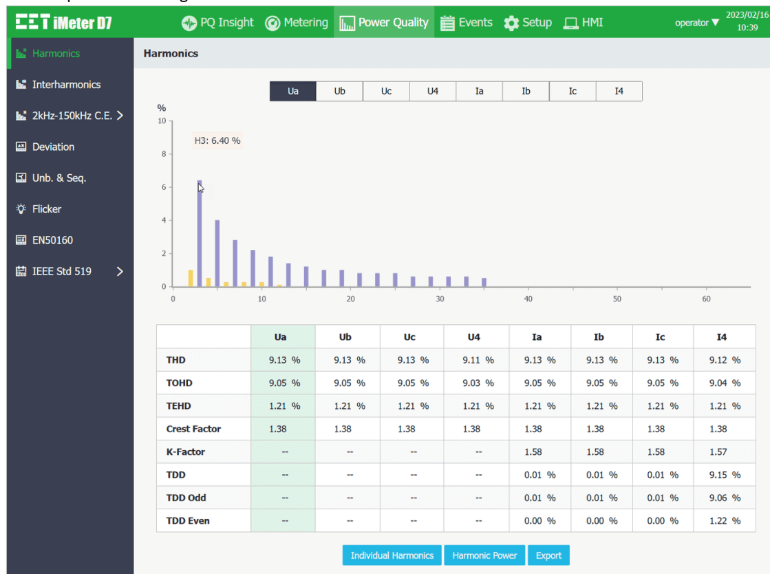
Figure 3-76 Harmonics Interface
