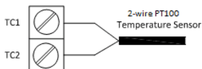
Figure 2-31 RTD Input Connections
