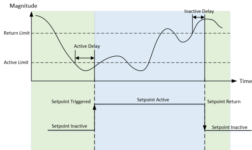
Figure 4-26 Under Setpoint
