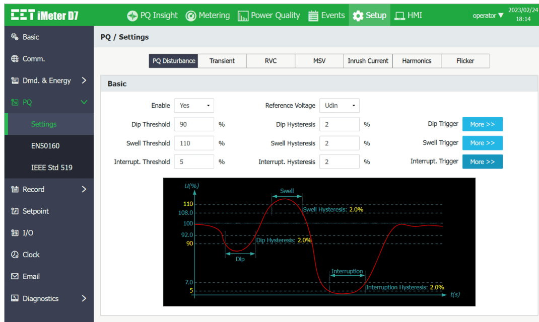
Figure 4-33 Setpoint Settings
