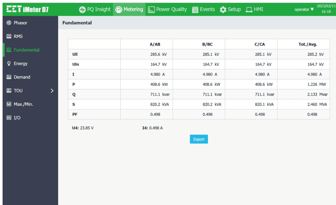
Figure 3-64 Fundamental Metering
