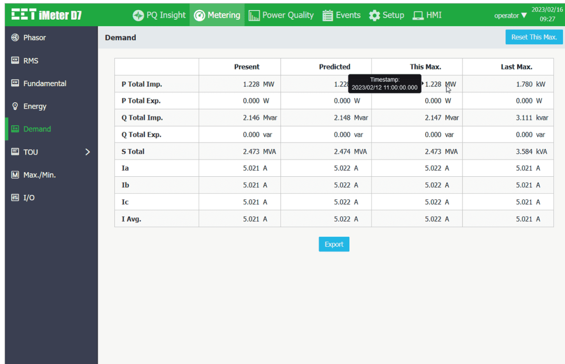
Figure 3-69 Demand Interface
