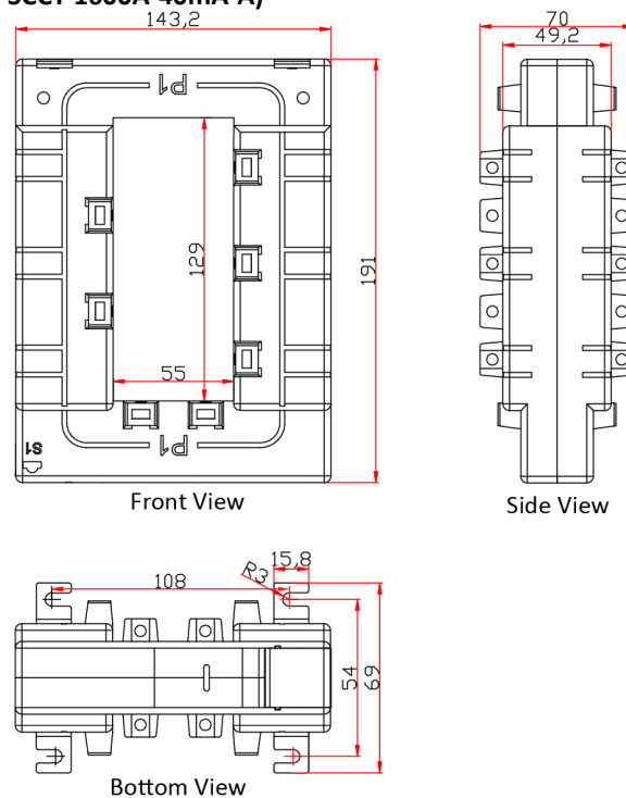
Figure 2-14 1600A Split Core CT Dimensions
