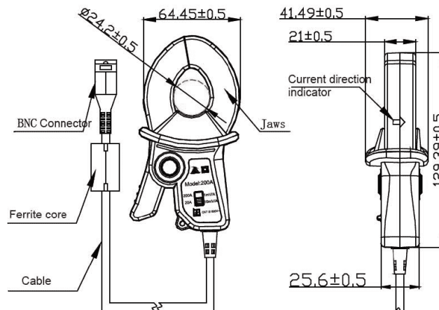
Figure 2-6 PMC-SCCP-200A-200mV-B-B-B Dimensions
