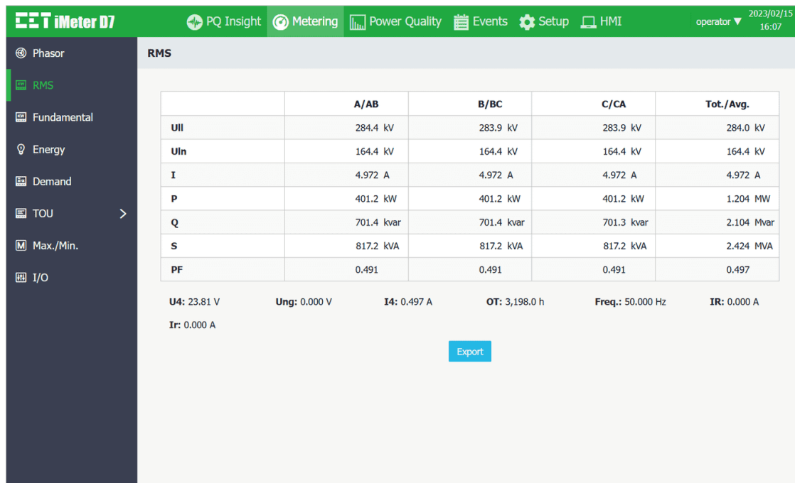
Figure 3-63 RMS Metering
