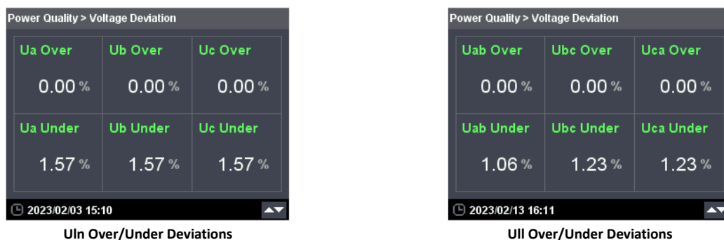
Figure 3-22 Voltage Deviation
