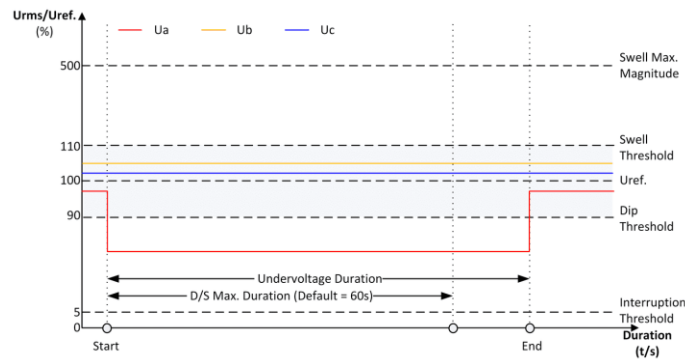
Figure 4-8 Undervoltage Detection Criteria
