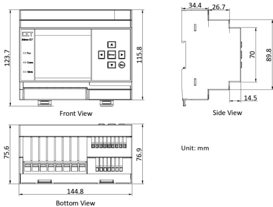
Figure 2-3 Dimensions
