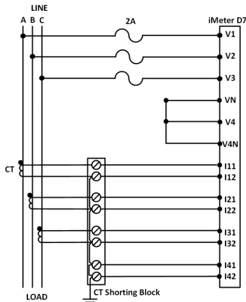
Figure 2-21 3-Phase 3-Wire Direct Delta Connection with 3CTs
