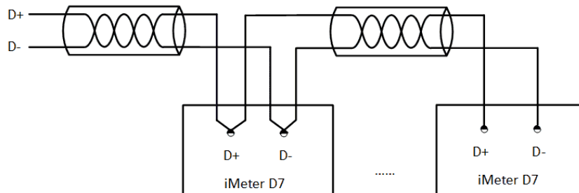
Figure 2-24 RS-485 Communication Connections
