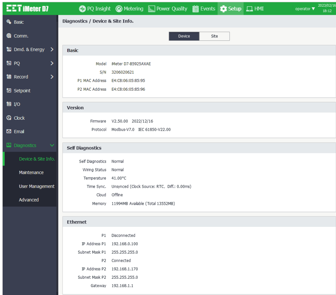
Figure 3-166 Device Info.
