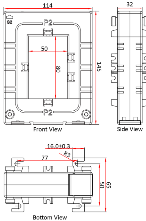
Figure 2-13 800A Split Core CT Dimensions
