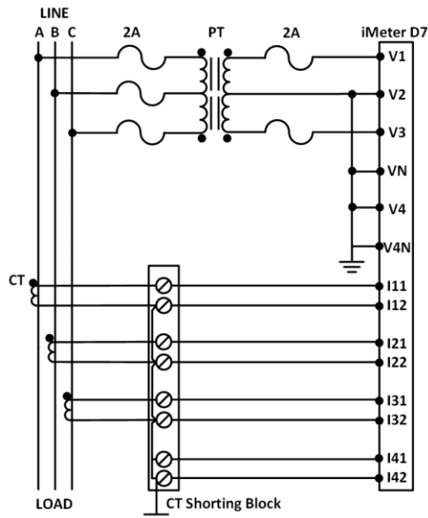
Figure 2-22 3-Phase 3-Wire Open Delta with 2PTs & 3CTs
