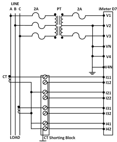
Figure 2-23 3-Phase 3-Wire Open Delta with 2PTs and 2CTs
