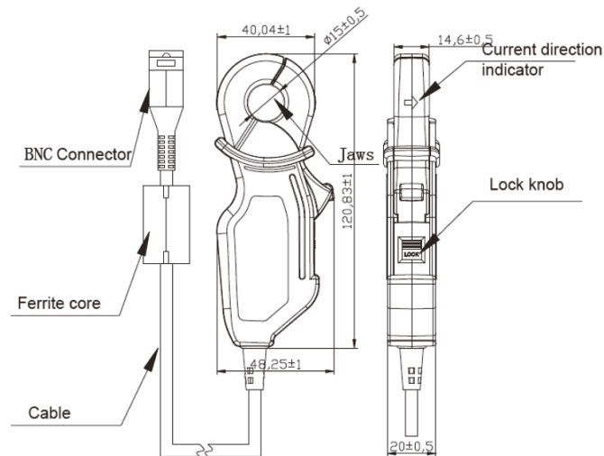
Figure 2-5 PMC-SCCP-50A-500mV-B-A-B Dimensions
