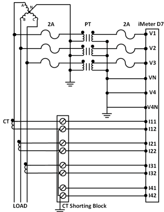
Figure 2-20 3-Phase 3-Wire Grounded Wye with 3PTs & 3CTs
