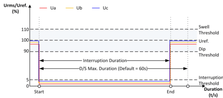
Figure 4-7 Interruption Detection Criteria
