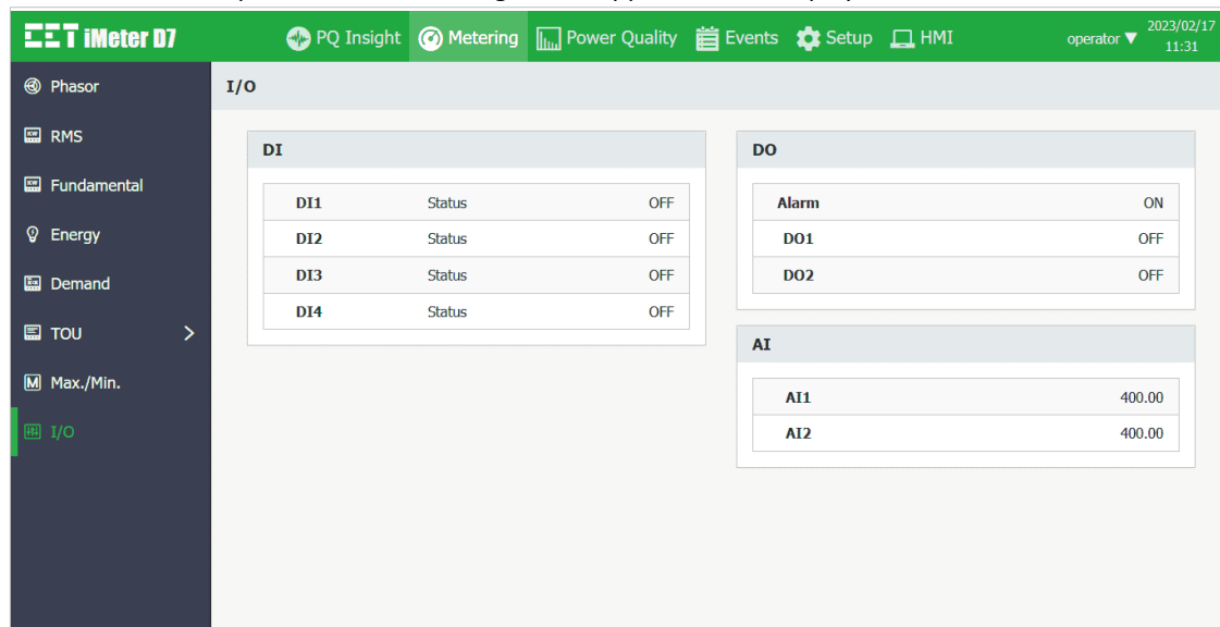
Figure 3-75 I/O Interface
