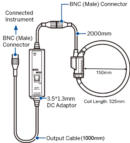
Figure 2-9 PMC-SCCP-5kA-500mV-B-C-C-150 Dimensions
