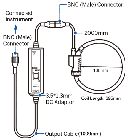
Figure 2-8 PMC-SCCP-5kA-500mV-B-C-C-100 Dimensions
