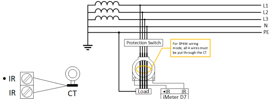
Figure 2-30 Residual Current Connections
