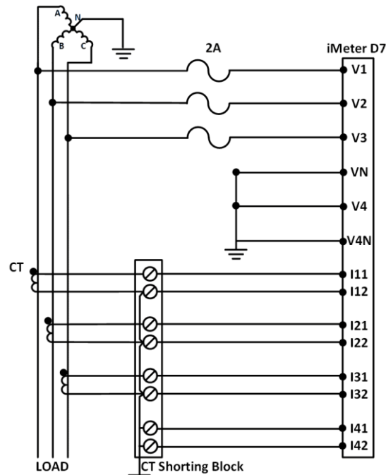
Figure 2-19 3-Phase 3-Wire Grounded Wye with no PTs & 3CTs
