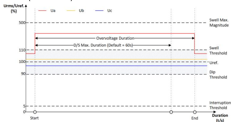
Figure 4-5 Overvoltage Detection Criteria 2
