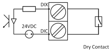
Figure 2-25 DI Connections
