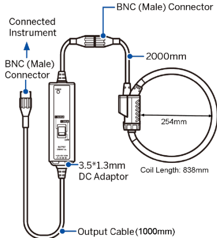
Figure 2-10 PMC-SCCP-5kA-500mV-B-C-C-254 Dimensions
