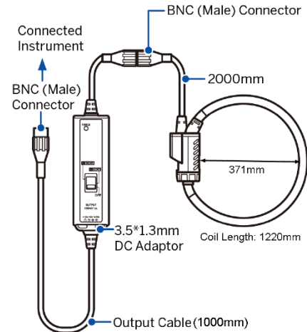
Figure 2-11 PMC-SCCP-5kA-500mV-B-C-C-371 Dimensions
