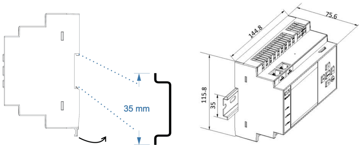
Figure 2-16 Installation
