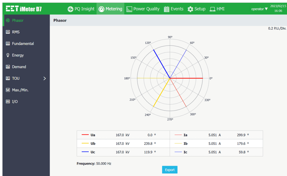
Figure 3-62 Phasor Diagram
