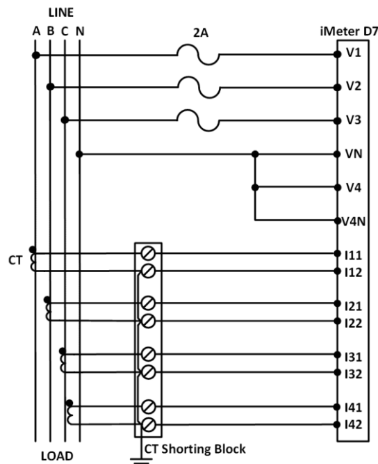
Figure 2-17 3-Phase 4-Wire Wye Direct Connection with 4CTs
