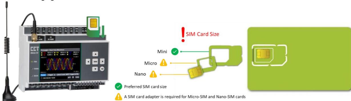
Figure 2-15 SIM Card Installation
