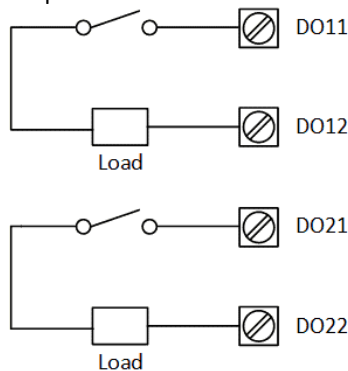
Figure 2-28 DO Connections
