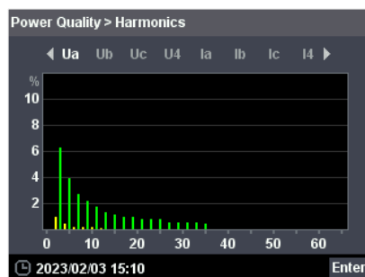
Harmonic Spectrum
