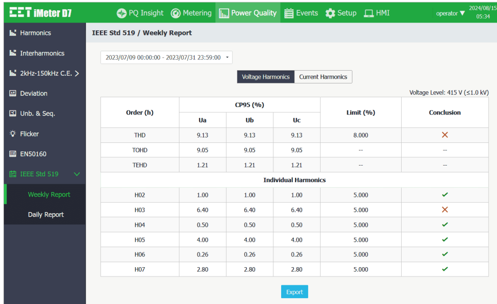
Figure 3-100 IEEE Std 519 Voltage Harmonics Compliance Weekly Report
