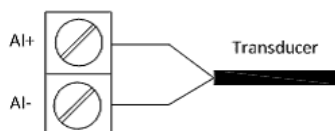
Figure 2-33 Analog Input Wiring
