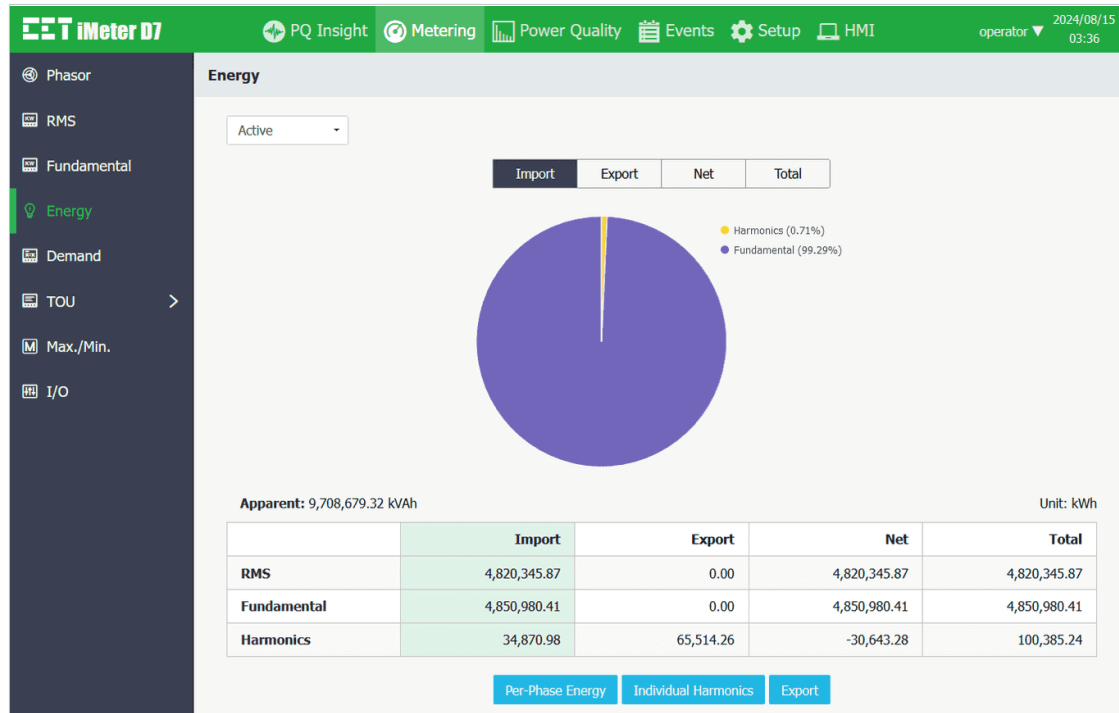
Figure 3-65 Energy Interface
