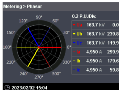
Figure 3-4 Phasor
