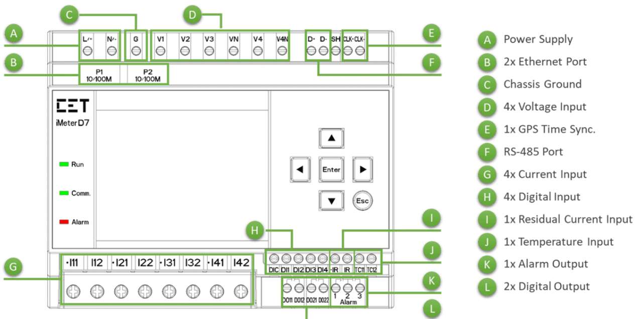
Figure 2-2 Terminals Diagram
