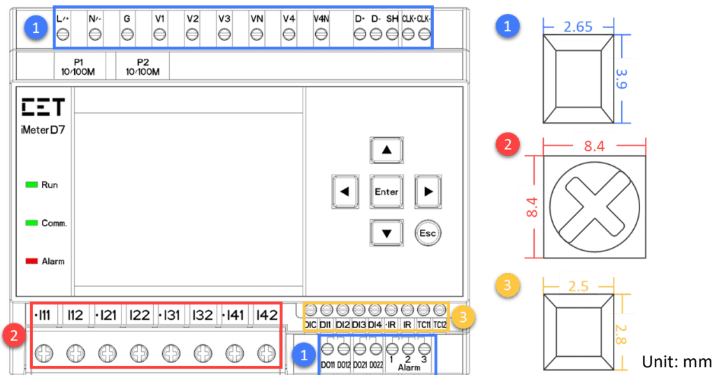
Figure 2-3 Dimensions
