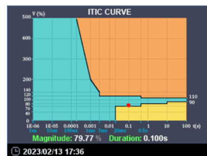
ITIC Curve
