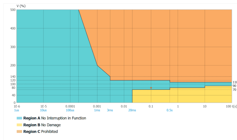
Figure 4-18 ITIC Plot Descriptions
