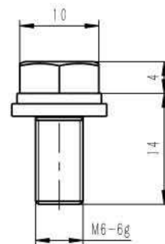
组合螺钉示意(选配) Combination Screw(Optional)
