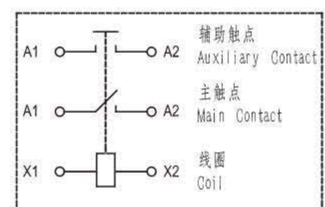
接线图 Coil Wiring Diagram
