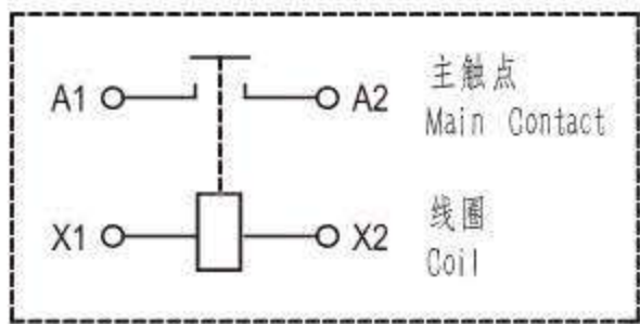
接线图 Coil Wiring Diagram
