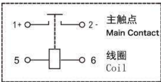
接线图 Coil Wiring Diagram
