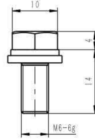
组合螺钉示意(选配) Combination Screw(Optional)
