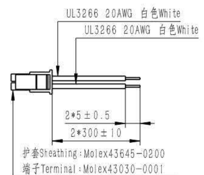
辅助触点连接器(选配) Auxiliary Contact Connector(Optional)
