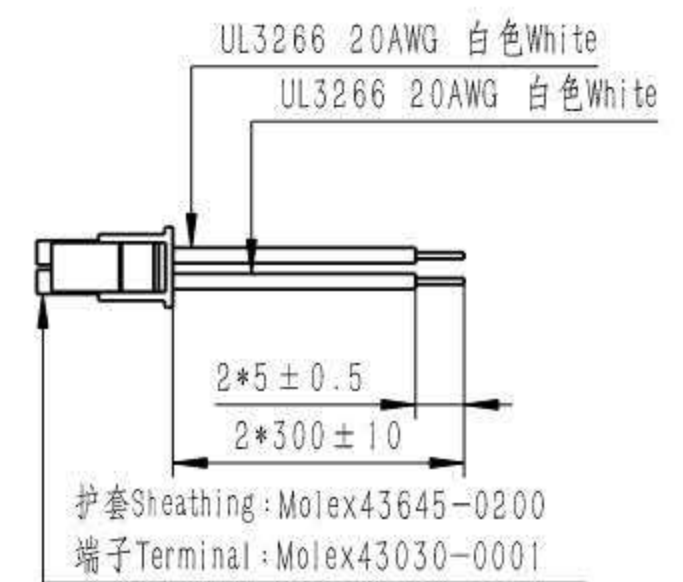
辅助触点连接器(选配) Auxiliary Contact Connector(Optional)
