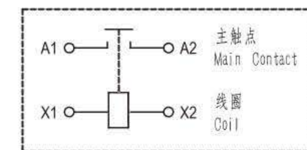
接线图 Coil Wiring Diagram
