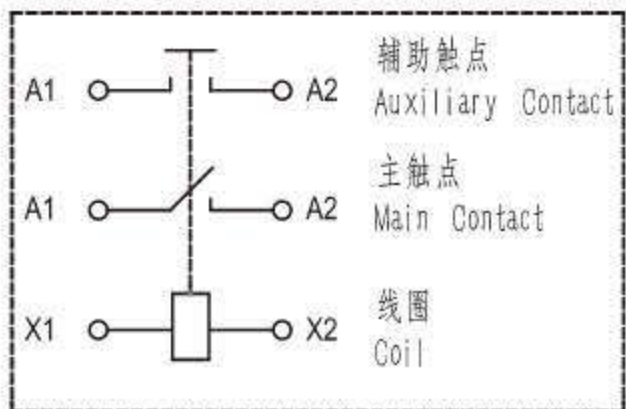
接线图 Coil Wiring Diagram 未注公差 General Tolerance: <10mm: ±0.3mm 10~50mm: ±0.5mm >50mm: ±0.8mm
