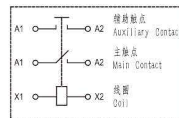
接线图 Coil Wiring Diagram
