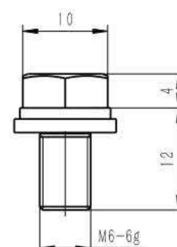
组合螺钉示意(选配) Combination Screw(Optional)
